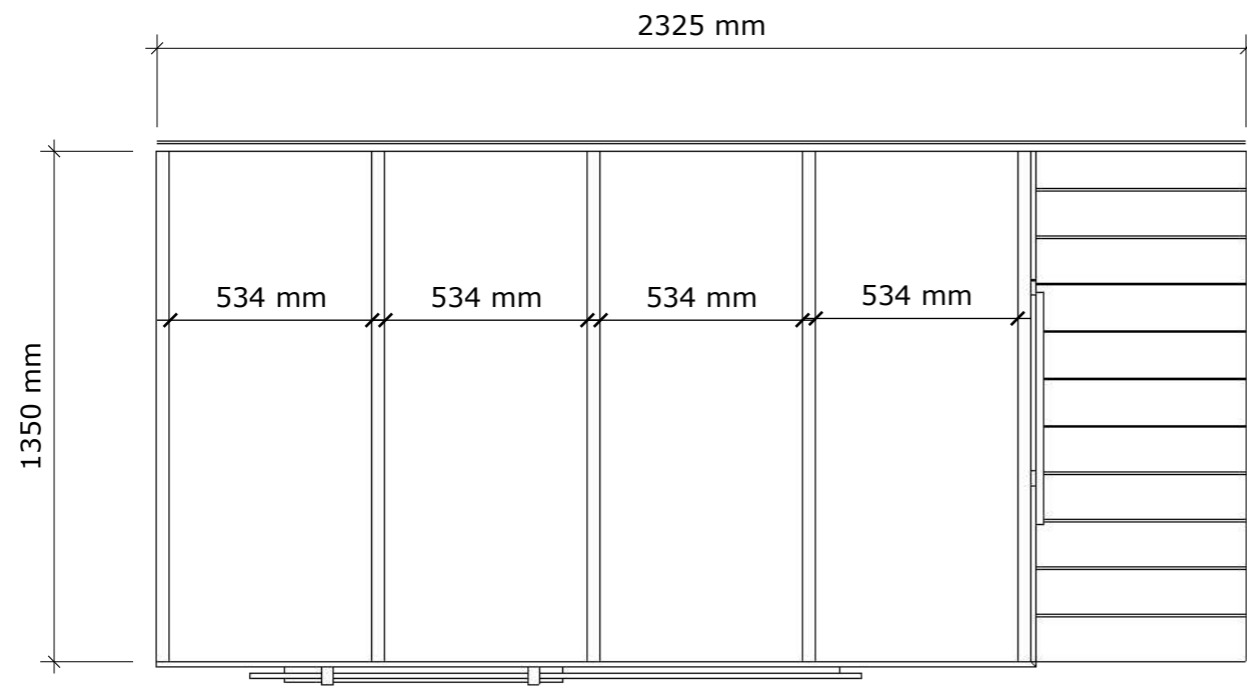
1 Plan Scale - 1:20
