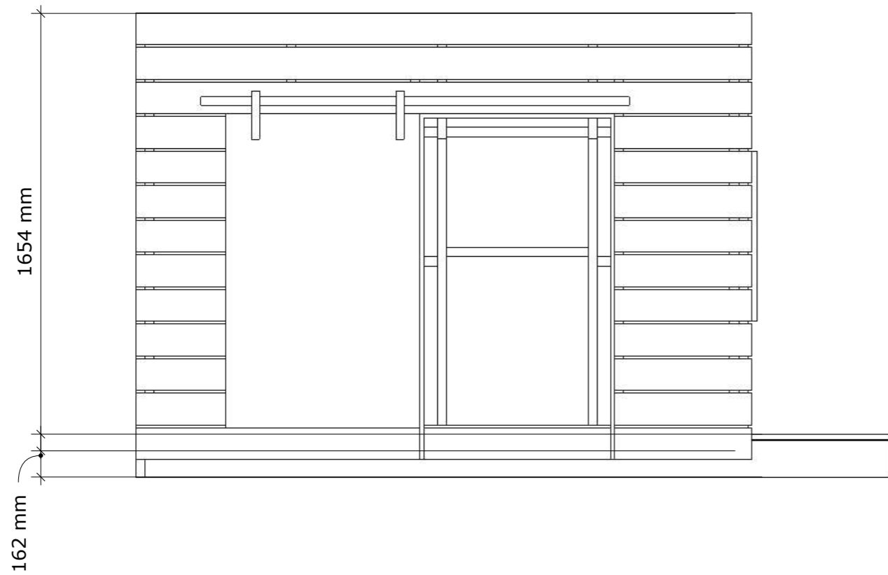
2 Elevation Scale - 1:20
