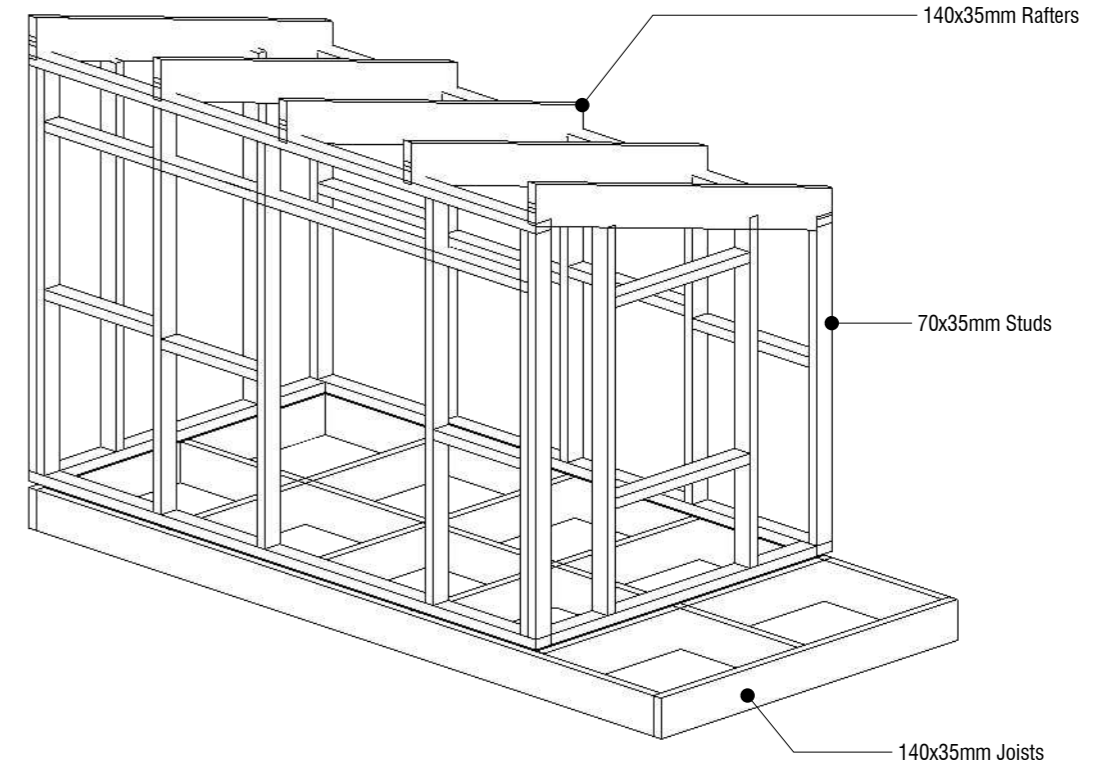
4 Axo - Framing Scale - 1:20
